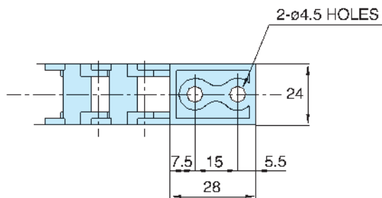
Moving Bracket
