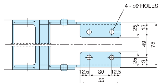
Moving Bracket
