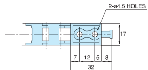
Moving Bracket
