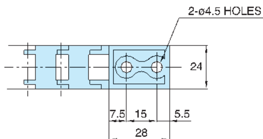
Fixed Bracket
