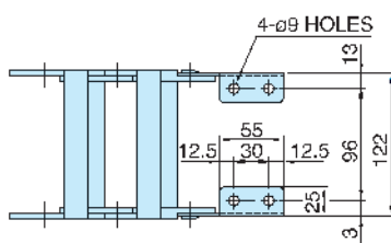
Fixed Bracket
