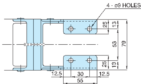
Fixed Bracket
