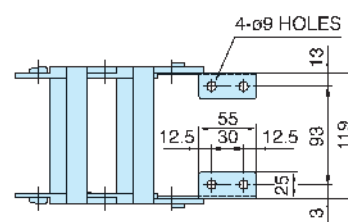
Moving Bracket
