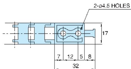
Fixed Bracket
