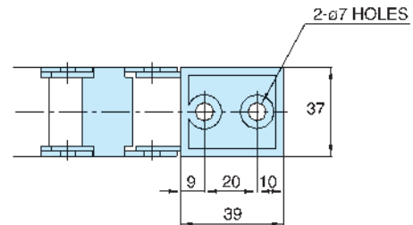
Moving Bracket
