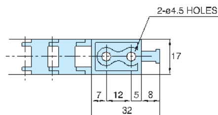
Fixed Bracket
