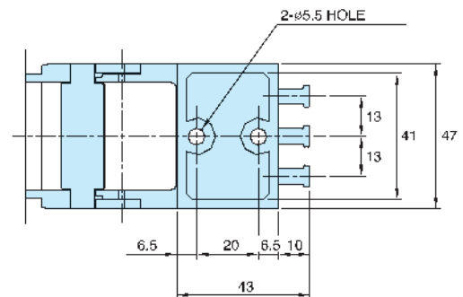
Moving Bracket
