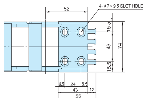
Moving Bracket
