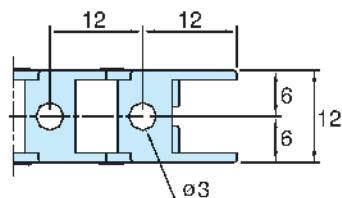
Fixed Bracket
