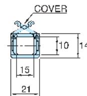
A-A Cross Section
