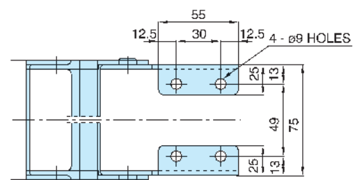
Moving Bracket
