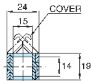
A-A Cross Section
