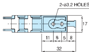
Moving Bracket
