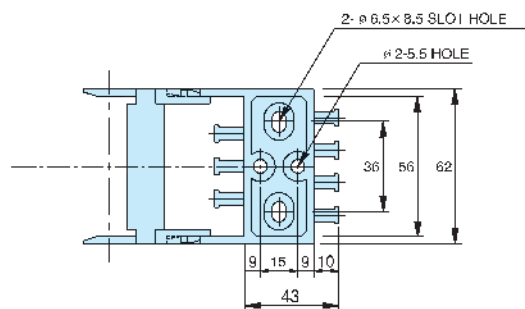
Fixed Bracket
