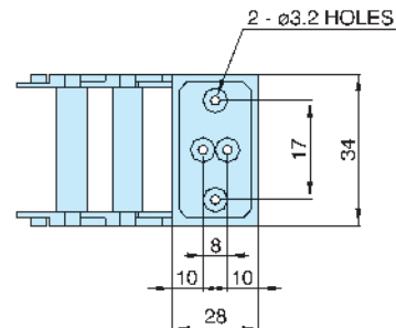
Moving Bracket
