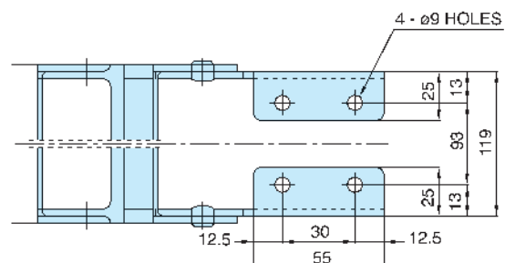
Moving Bracket
