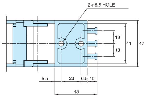
Fixed Bracket
