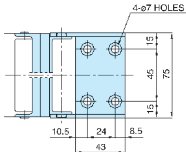
Fixed Bracket
