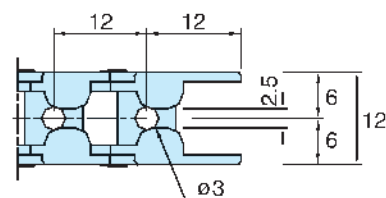
Moving Bracket
