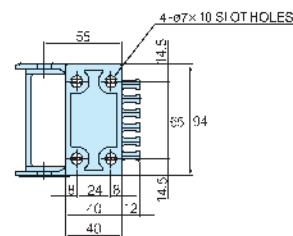
Moving Bracket
