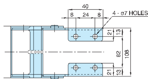
Moving Bracket
