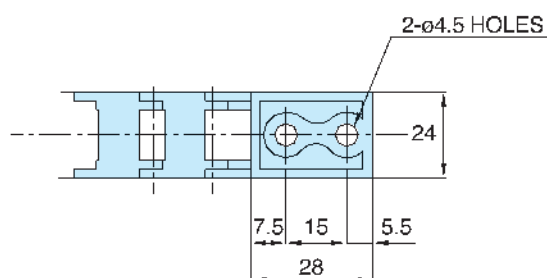
Moving Bracket
