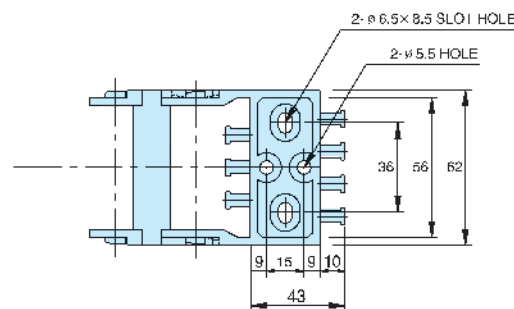
Moving Bracket
