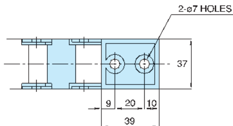
Fixed Bracket
