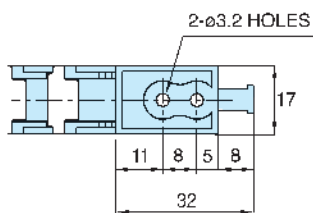
Fixed Bracket
